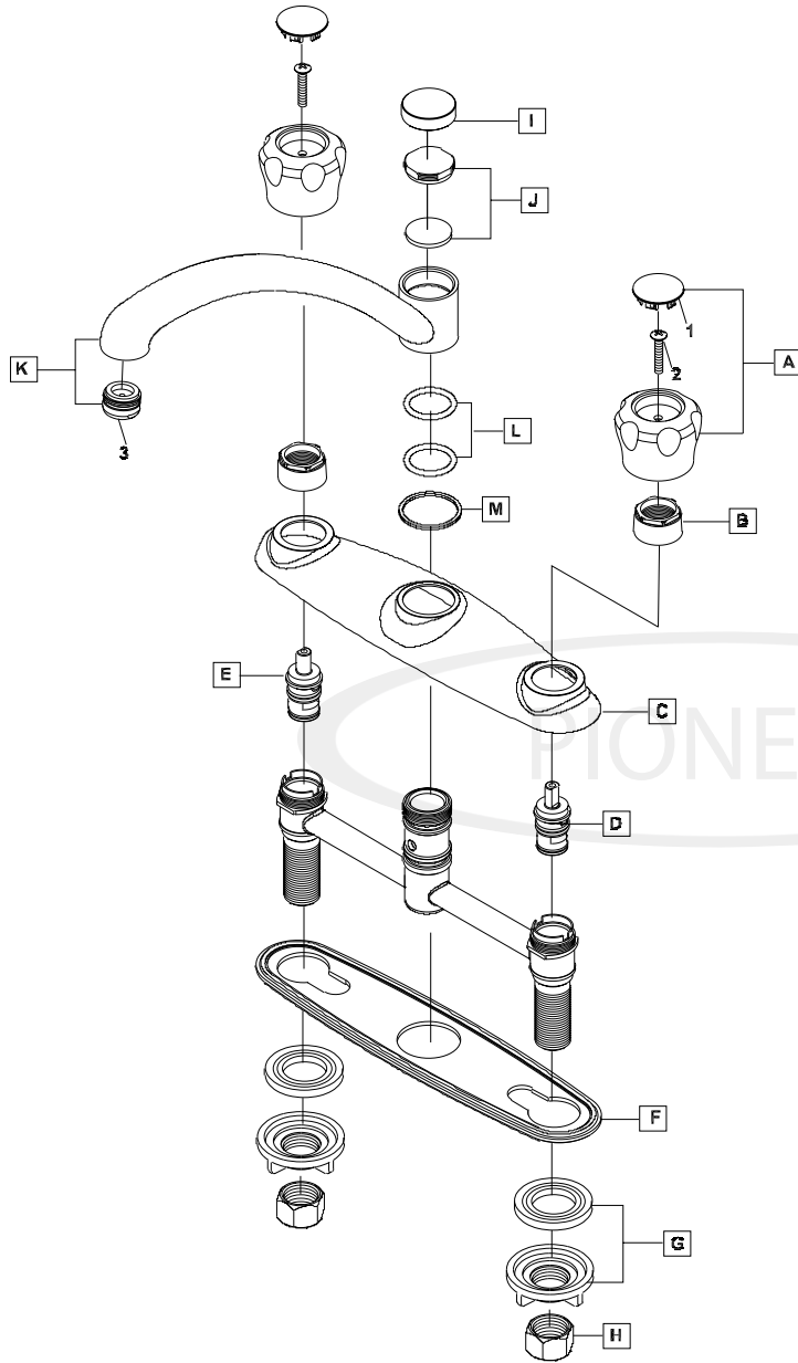
Product Diagram
